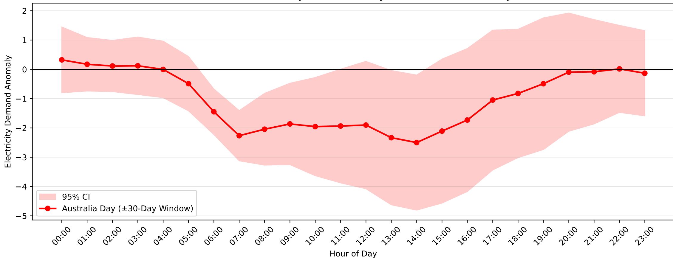
Rutherford Demand Anomaly: Australia Day (2004-2017, \pm 30 -Day Window)
